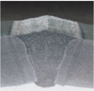
MIG-MAG
